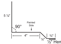
7. Sidewall Flashing
