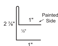
23. "F" Channel
