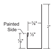
9. "J" Channel
