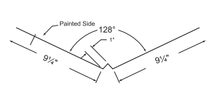
4. W-Valley
