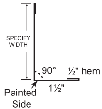
13. Fascia Trim
