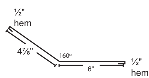
11A. Transition
