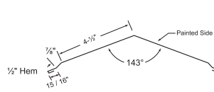
3. Ridge Cap
